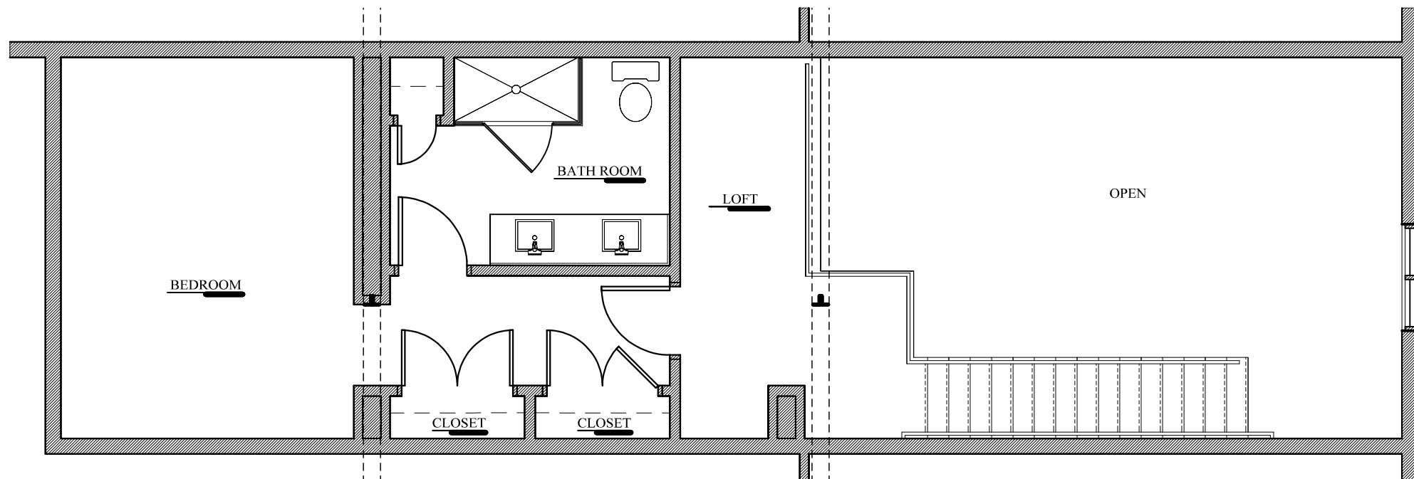
LOFT LEVEL (UNIT #8) (485 SQ. FT.)
