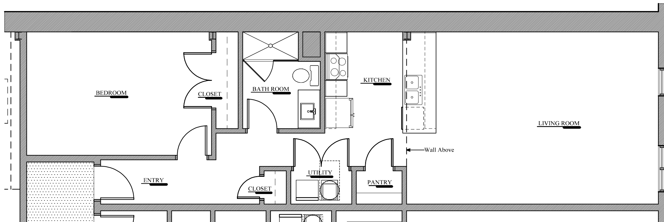
FIRST FLOOR (UNIT #7) (880 SQ. FT.)
