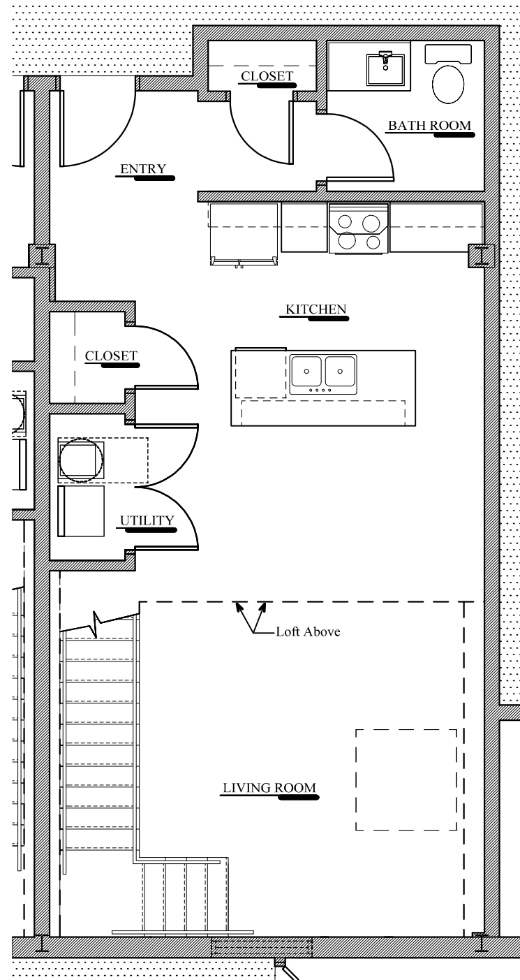
FIRST FLOOR (UNIT #5) 0 2 4 8 (630 SQ. FT.)
