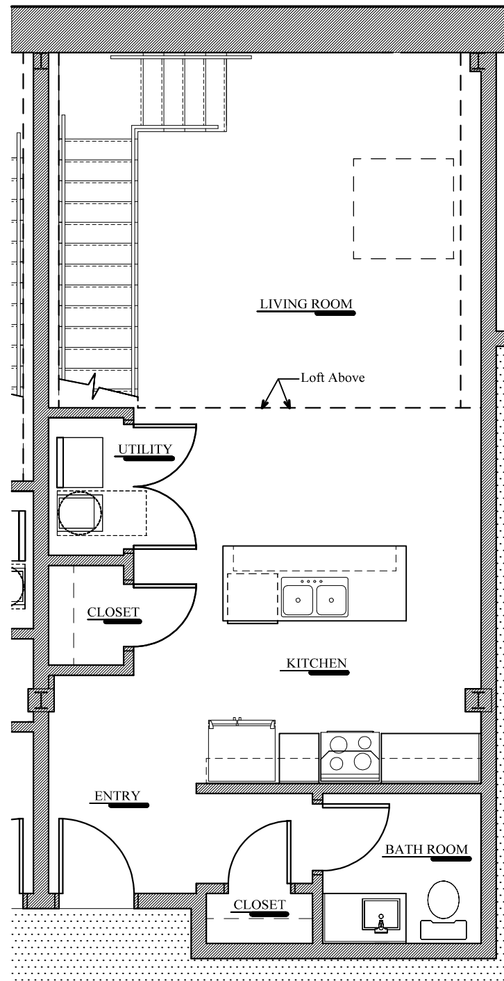
FIRST FLOOR (UNIT #3) 0 2 4 8 (630 SQ. FT.)
