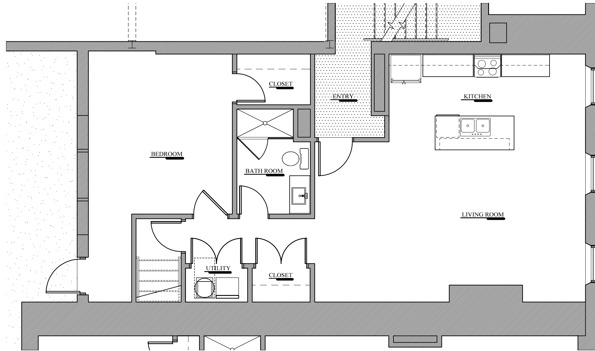
FLOOR PLAN (UNIT #22) (902 SQ. FT.)
