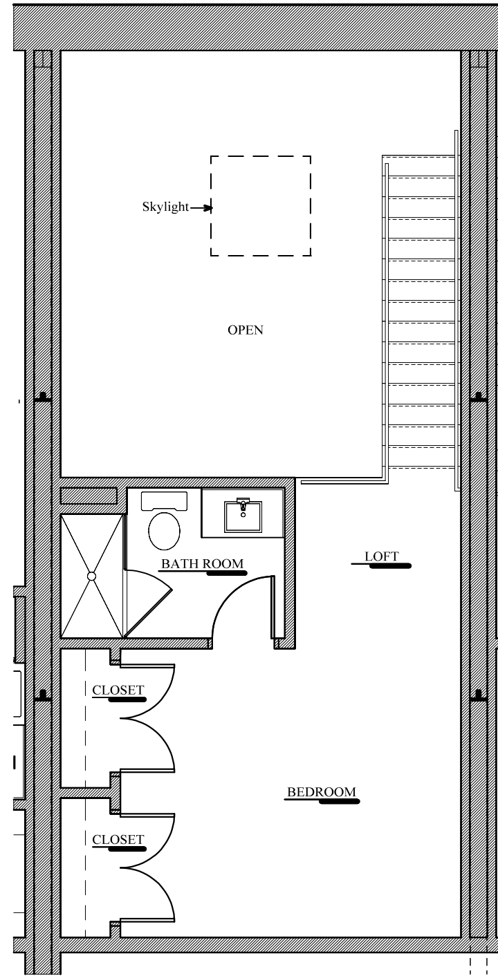
LOFT LEVEL (UNIT #2) (329 SQ. FT.)
