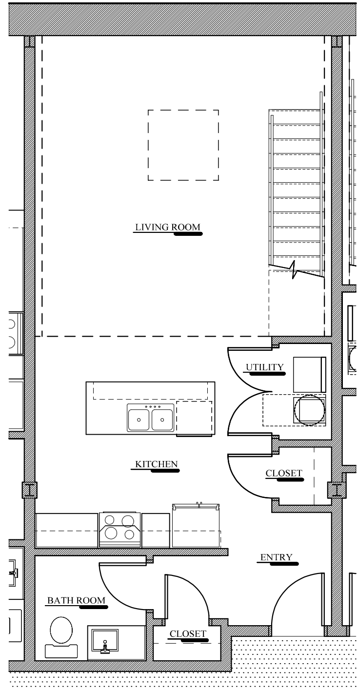
FIRST FLOOR (UNIT #2) (616 SQ. FT.)
