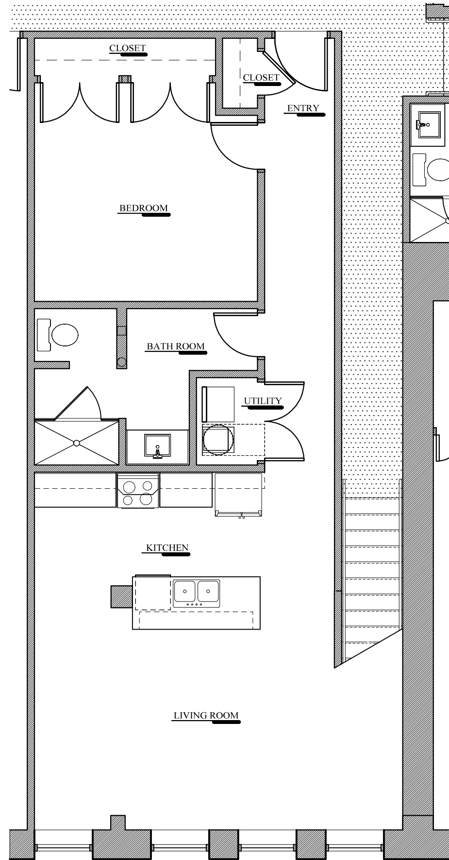
FLOOR PLAN (UNIT #15) (835 SQ. FT.)
