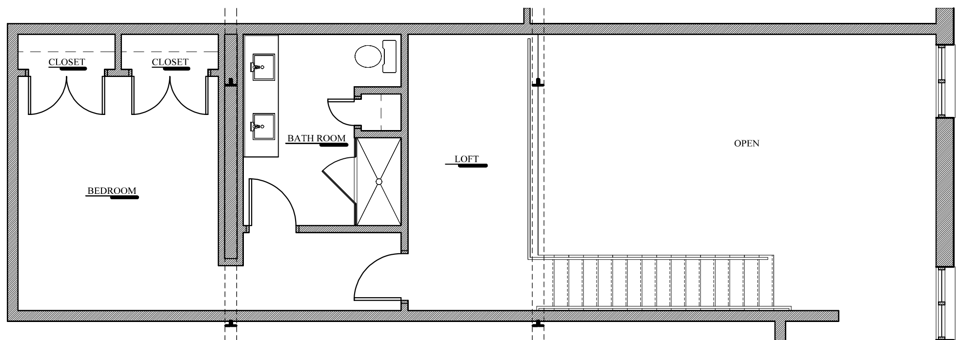
LOFT LEVEL (UNIT #10) (490 SQ. FT.)
