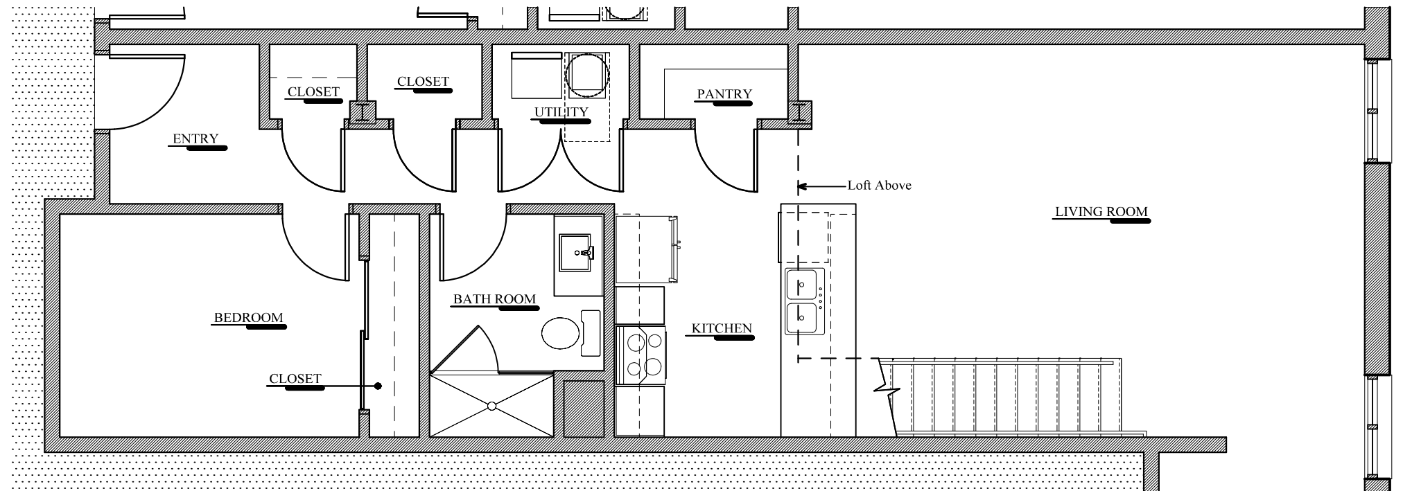
FIRST FLOOR (UNIT #10) (965 SQ. FT.)
