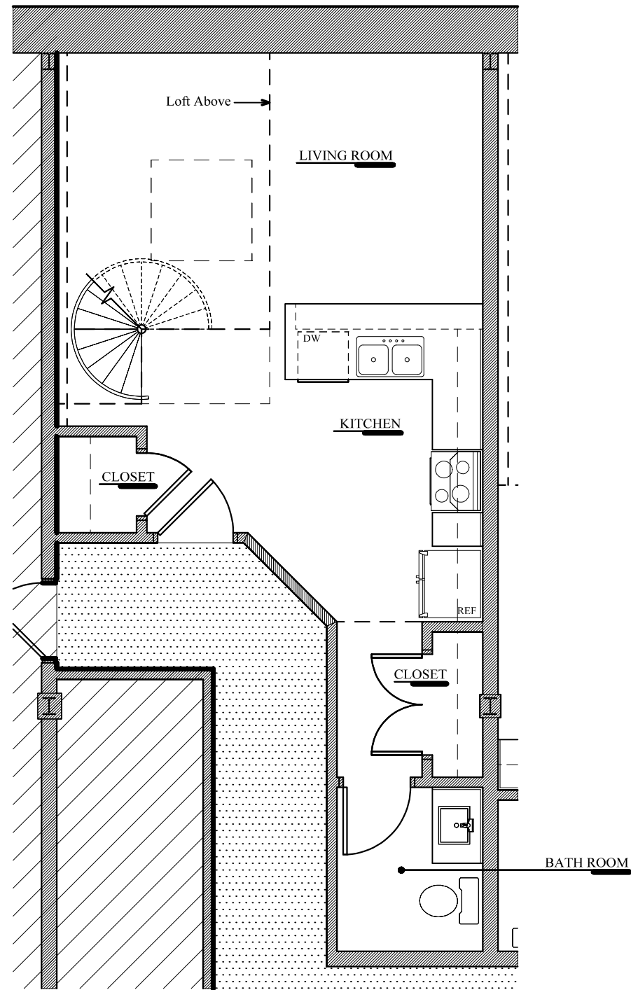
FIRST FLOOR (UNIT #1) 0 2 4 8 (448 SQ. FT.)
